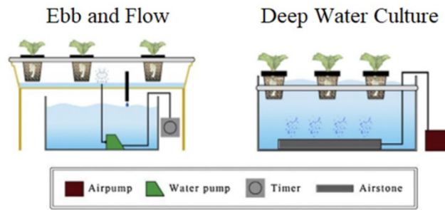
Figure 2: Ebb and flow (left) and deep water culture (right) hydroponic systems. Adapted from Lee and Lee (2015)(Lee & Lee, 2015).
