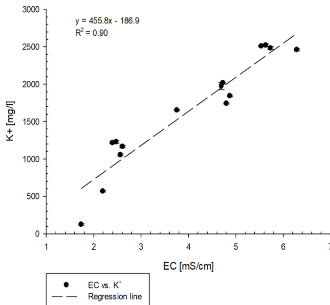
Figure 36: Electrical conductivity vs. Potassium: Scatter plot and fitted linear regression line with formula for potassium ( K^+ ) as dependent and electrical conductivity (EC) as explanatory variable.
