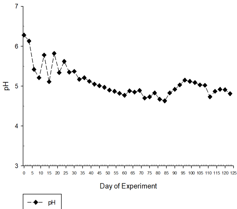
Figure 29: pH development of the Phosphorus Reactor.
