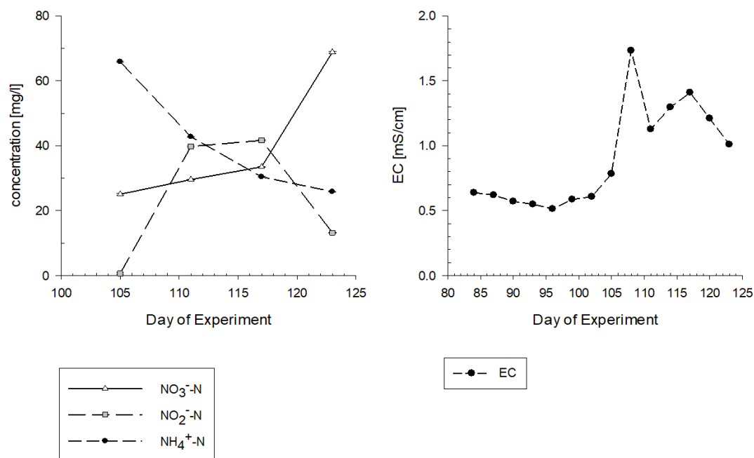
Figure 27: Nutrient and electrical conductivity (EC) concentration development of Nitrate Reactor II. Ammonium nitrogen ( \text{NH}_4^+ -N), nitrite nitrogen ( \text{NO}_2^- -N), and nitrate nitrogen ( \text{NO}_3^- -N) concentrations (left) from day of experiment 105, as the transfer of \text{NH}_4^+ rich solution started and EC (right), measured from the starting day of the reactor.
