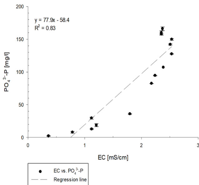
Figure 31: Electrical conductivity (EC) vs. phosphate phosphorus ( \text{PO}_4^{3-}\text{-P} ): Scatter plot and fitted linear regression line with formula for \text{PO}_4^{3-}\text{-P} as dependent and EC as explanatory variable.
