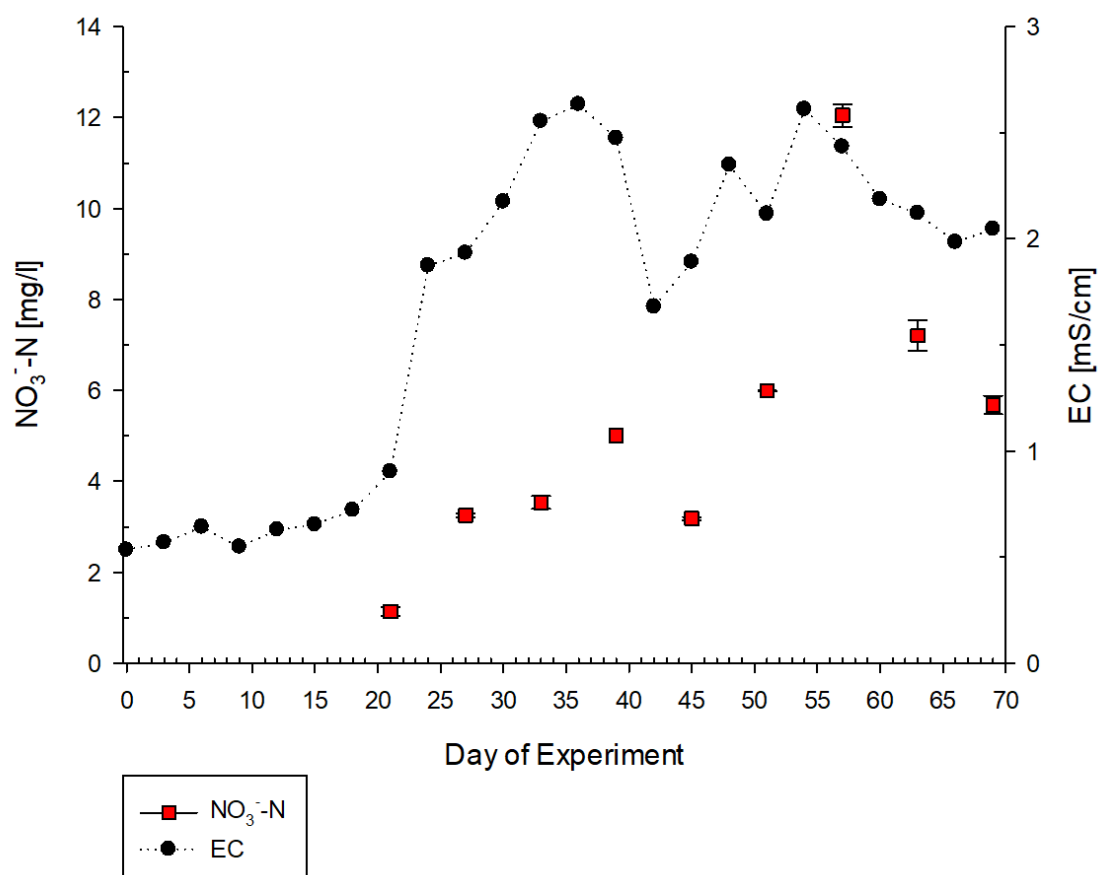
Figure 26: Nitrate Reactor I: Nitrate nitrogen ( \text{NO}_3^- -N) and electrical conductivity (EC) concentration development.
