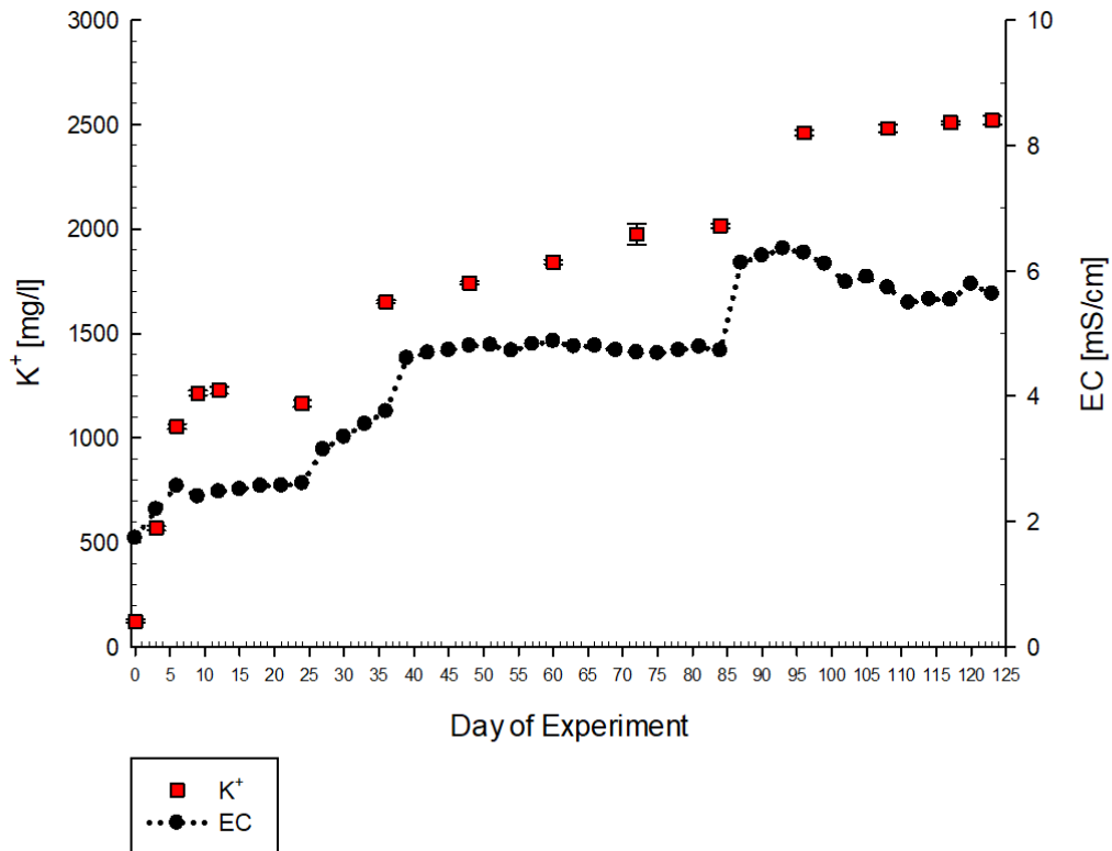
Figure 35: Potassium Reactor: Potassium ( K^+ ) and electrical conductivity (EC) concentration development.
