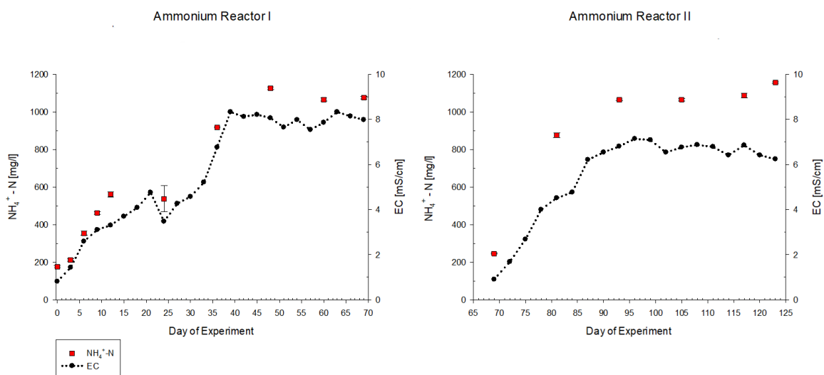
Figure 21: Ammonium-Reactors: Ammonium nitrogen ( \text{NH}_4^+ -N) and electrical conductivity (EC) concentration development of the two time-shifted ammonium reactors. Ammonium Reactor I (left) and Ammonium Reactor II (right).
