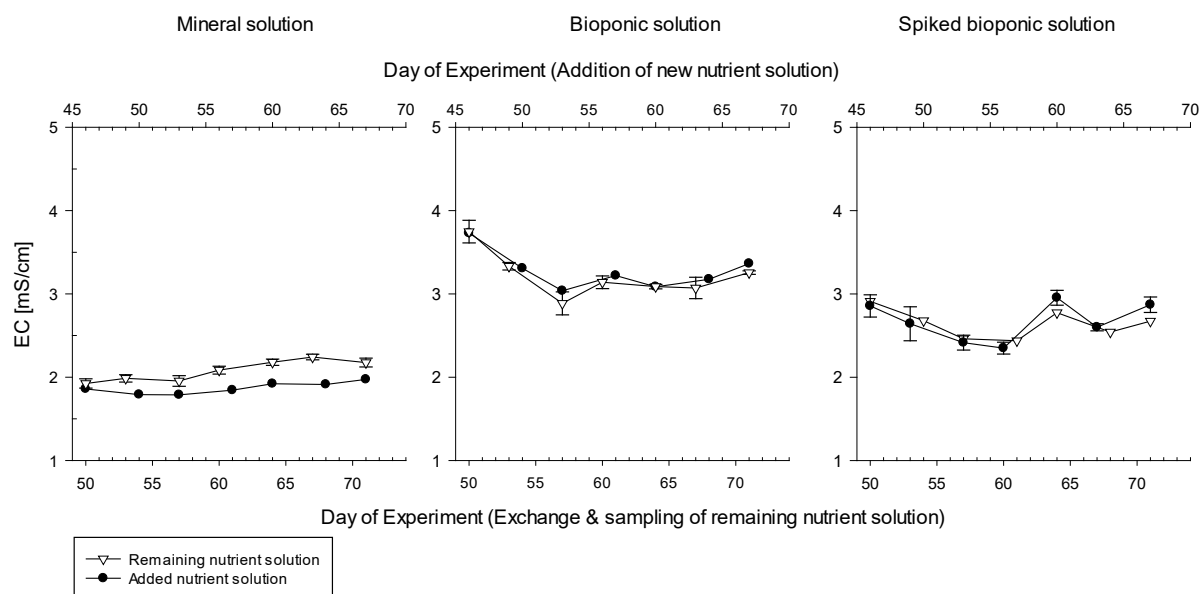
Figure 39: Electrical Conductivity (EC) of added and remaining nutrient solution in the deep-water culture containers after intervals of three or four days for each tested solution. Days nutrient solution was added are shown on the upper x-axis. "Added nutrient solution" refers to this axis. Days the nutrient solution was exchanged and sampled are shown on the lower x-axis, "Remaining nutrient solution" refers to this axis.
