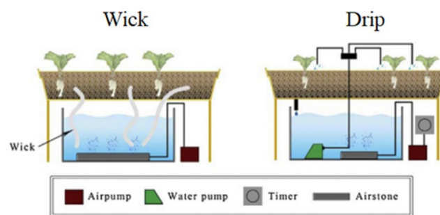
Figure 1: Wick (left) and drip irrigation (right) hydroponic systems. Adapted from Lee and Lee (2015).
