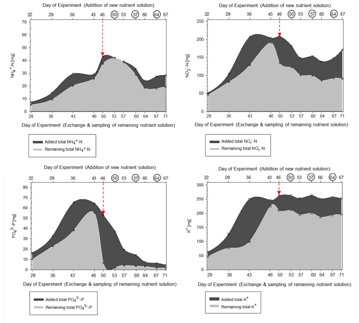
Figure 51: Added and remaining nutrient masses of the spiked bioponic solution. Days nutrient solution was added are shown on the upper x-axis; added nutrient mass refers to this axis. Days the nutrient solution was exchanged and sampled are shown on the lower x-axis; remaining nutrient mass refers to this axis. Stacked symbols (x) represent the added and remaining mass of nutrients within an interval of three or four days. The difference between two symbols corresponds to the nutrient uptake by the plant. The red dotted arrow marks the start of the comparison phase and the added nutrient mass on that day. For presentation reasons, no linear axis labels were selected. All values are mean values ( n=4 ); no standard deviation was included for presentation reasons. Circled days represent days added nutrient mass was calculated by means.
