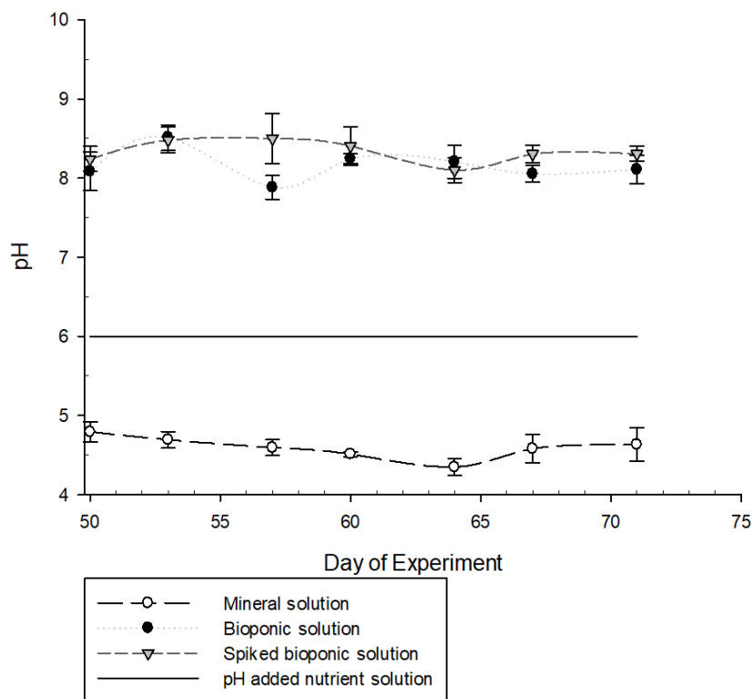
Figure 38: pH of the nutrient solutions on exchange days after three or four days in the deep-water culture containers.
