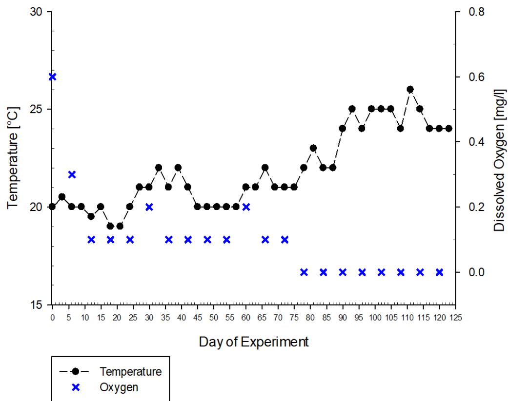
Figure 33: Potassium Reactor: Temperature and dissolved oxygen concentration development.
