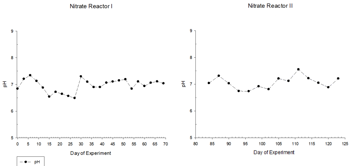
Figure 25: pH development of the two time-shifted nitrate reactors. Nitrate Reactor I (left) and Nitrate Reactor II (right).
