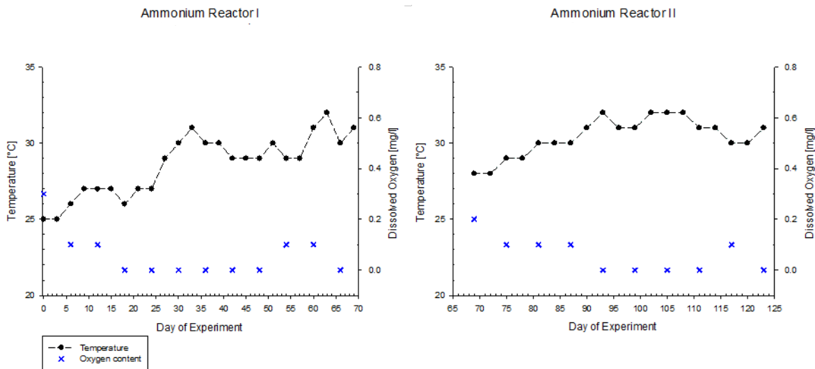
Figure 19: Ammonium-Reactors: Temperature and dissolved oxygen concentration development of the two time-shifted ammonium reactors. Ammonium Reactor I (left) and Ammonium Reactor II (right).
