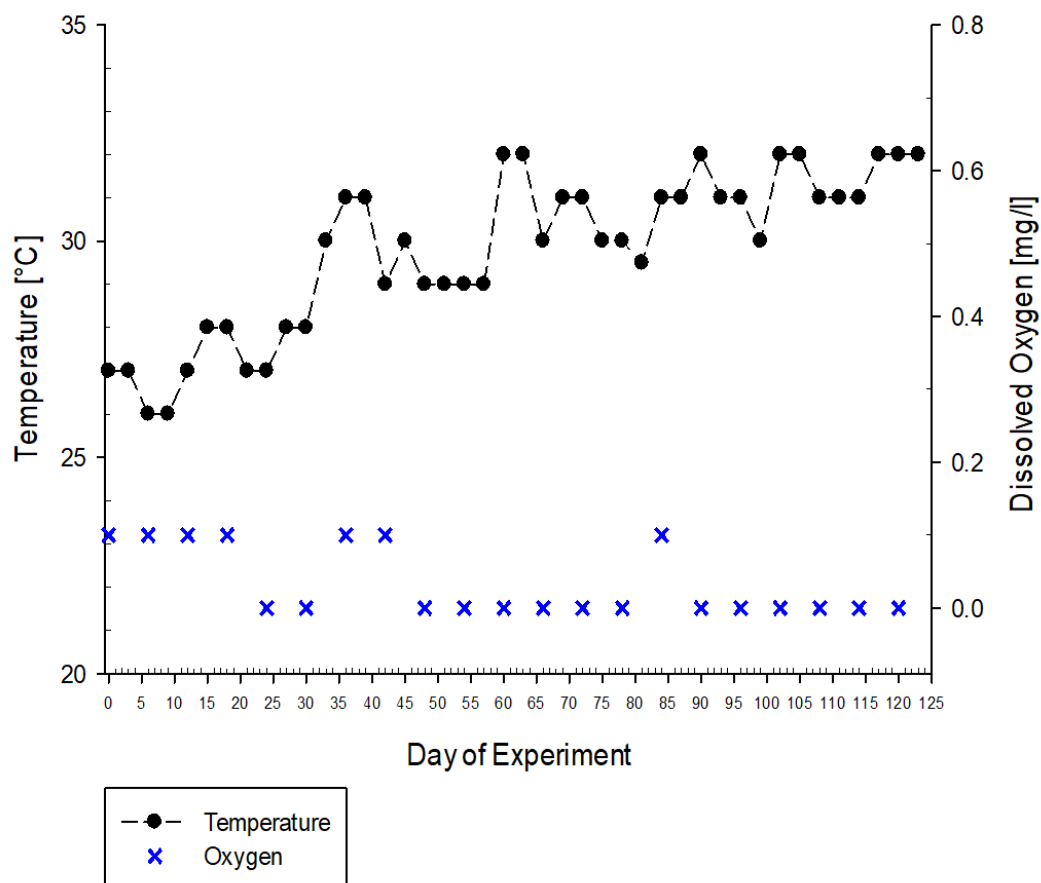
Figure 28: Phosphorus Reactor: Temperature and dissolved oxygen concentration development.
