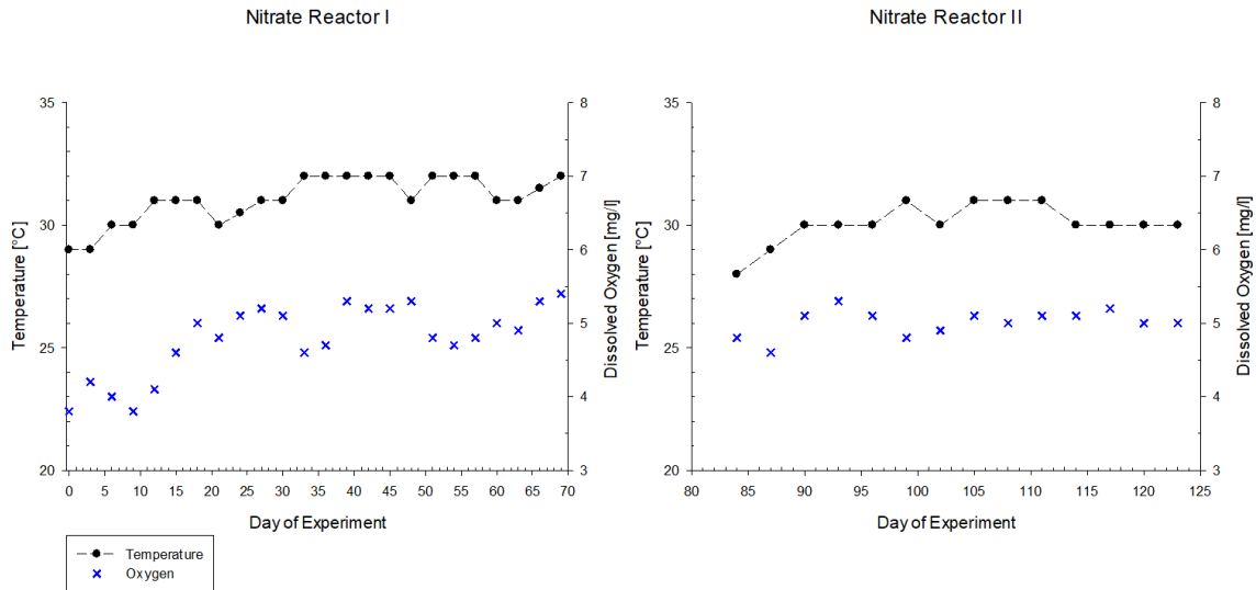
Figure 24: Nitrate-Reactors: Temperature and dissolved oxygen concentration development of the two time-shifted nitrate reactors. Nitrate Reactor I (left) and Nitrate Reactor II (right).
