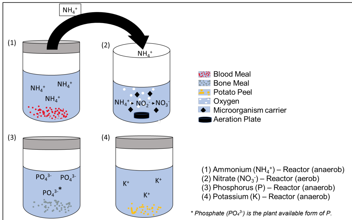
Figure 8: Graphical illustration of the four reactors and the process of ammonium-rich solution transfer into the aerated nitrate reactor for nitrification.
