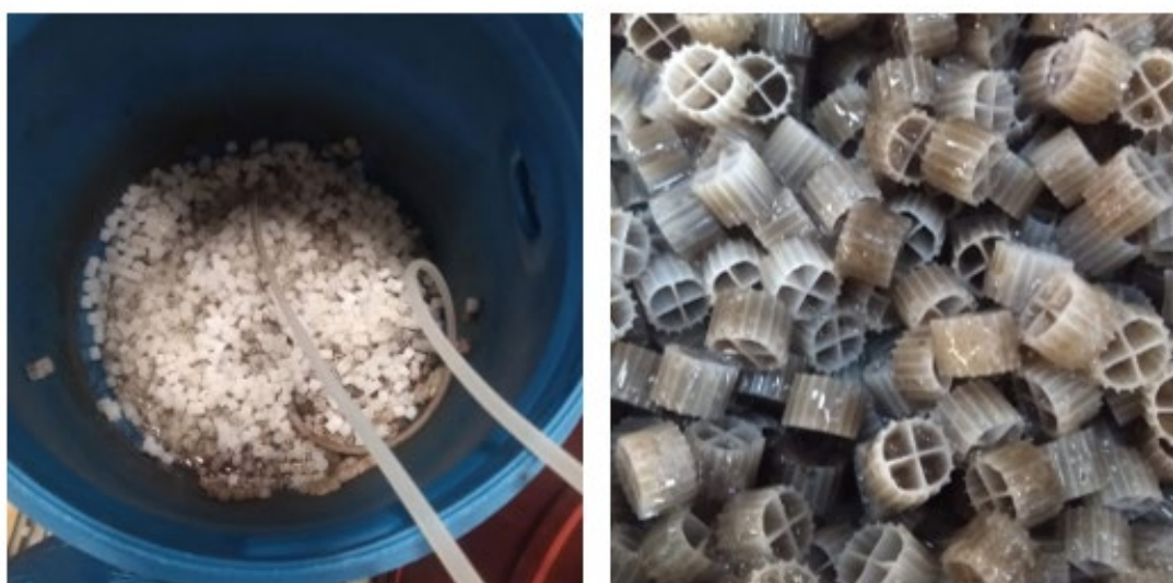
Figure 11: Microorganism carriers: During the start phase for inoculation (left). Inoculated Microorganism carriers (right), as transferred into the NO 3 - -Reactor .
