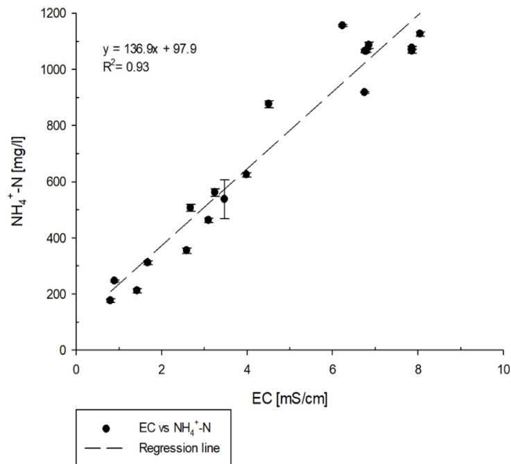
Figure 22: Electrical conductivity (EC) vs. ammonium nitrogen ( \text{NH}_4^+\text{-N} ): Scatter plot and fitted linear regression line with formula for \text{NH}_4^+\text{-N} as dependent and EC as explanatory variable.
